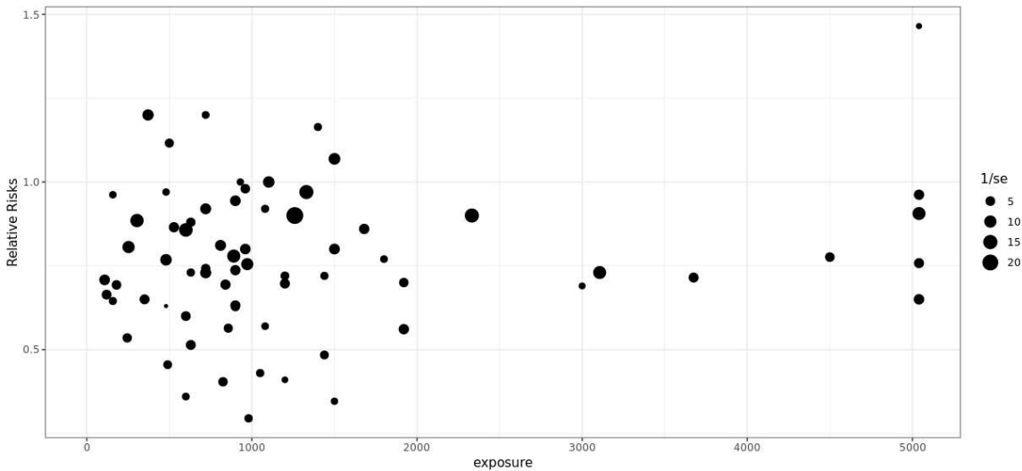
Scatter plot of RRs vs original exposure variable
